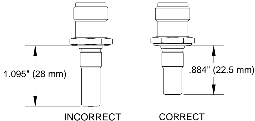
Figure 1. Igniter dimensions
