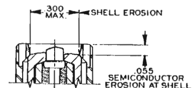
WORN OUT
