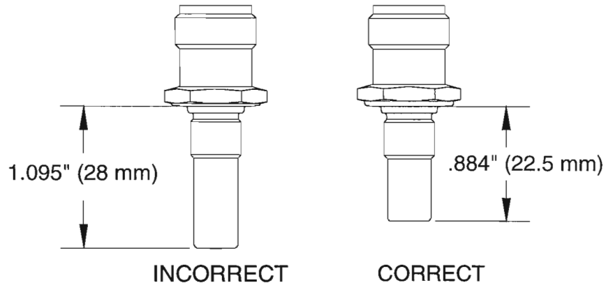
Figure 1. Igniter Dimensions.
